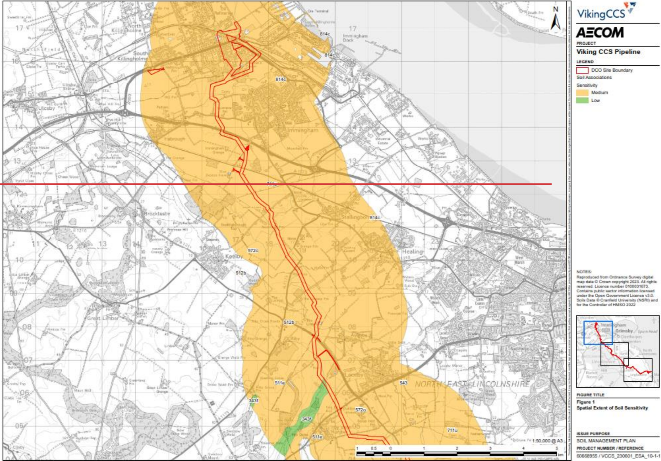
Figure 1: Spatial Extent of Soil Sensitivity
