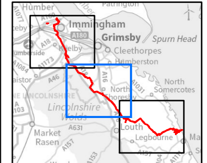
FIGURE TITLE Figure 1 Spatial Extent of Soil Sensitivity
